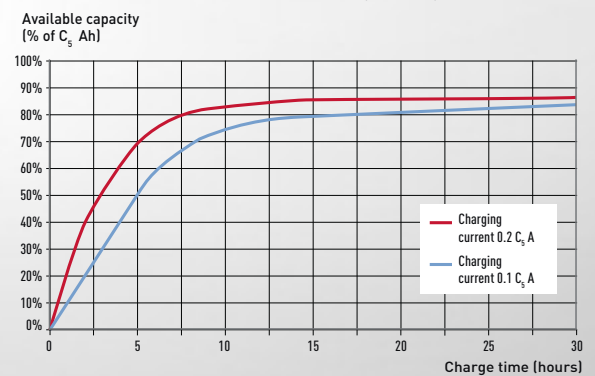
SBM Range – Available capacity after constant voltage charge 1.40 VPC at + 20°C (+ 68°F)
